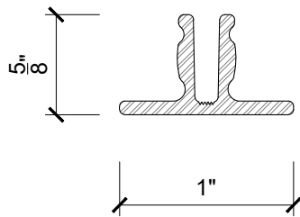
1 PL10 (TRIM) - PROFILE PL10-A SCALE 1'-0"=1'-0"
