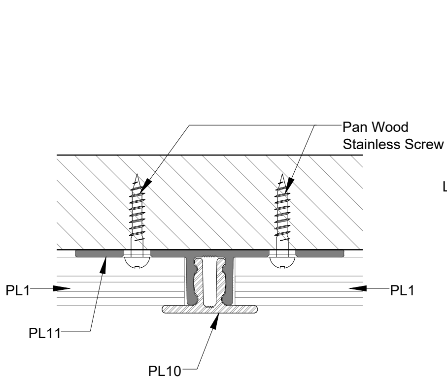
1 PL10 (TRIM) - APPLICATION PL10-B SCALE 1'-0"=1'-0"
