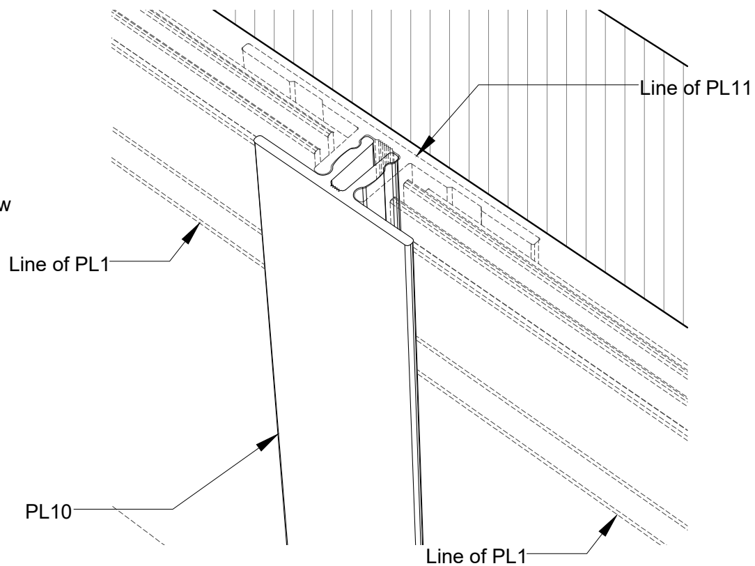
2 PL10 (TRIM) - APPLICATION - 3D VIEW PL10-B SCALE NTS
