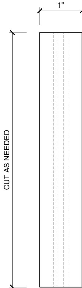
2 PL10 (TRIM) - FRONT PL10-A SCALE 9"=1'-0"
