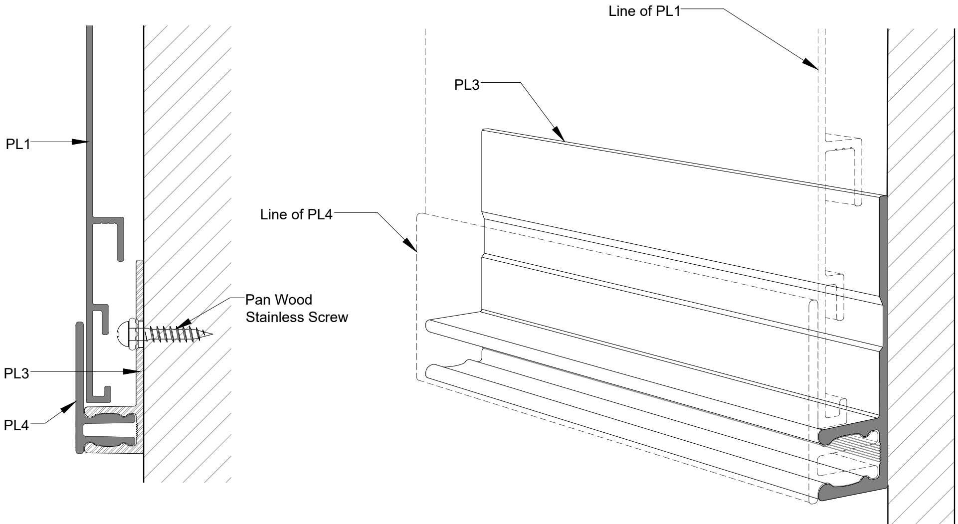
1 PL3 - APPLICATION PL3-B SCALE 1'-0"=1'-0"
