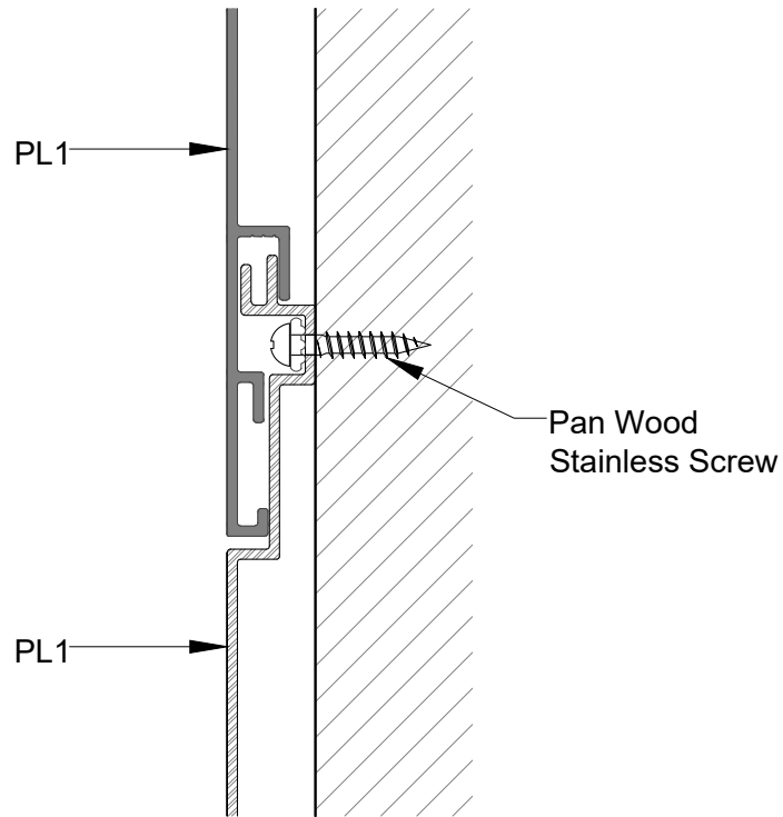
1 PL1 - APPLICATION (BUTT JOIN) PL1-C SCALE 9"=1'-0"
