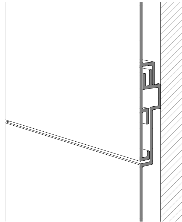
2 PL1 - APPLICATION (BUTT JOIN) - 3D VIEW PL1-C SCALE NTS
