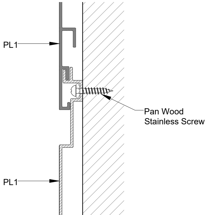
1 PL1 - APPLICATION (SHIPLAP) PL1-D SCALE 9"=1'-0"
