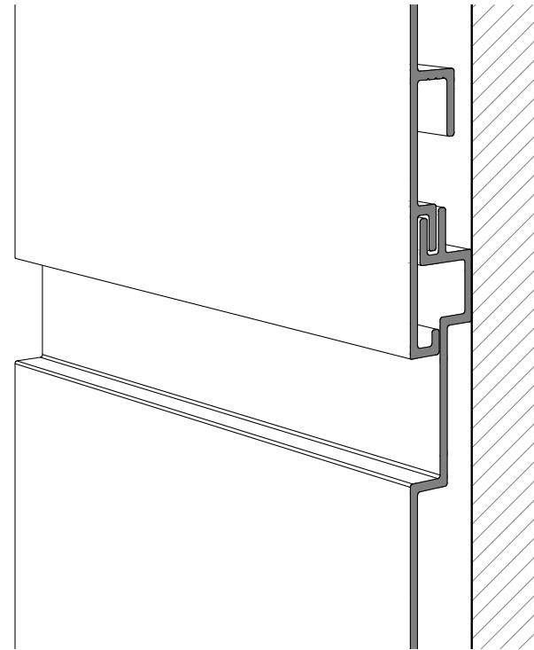
2 PL1 - APPLICATION (SHIPLAP) - 3D VIEW PL1-D SCALE NTS
